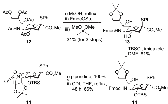
Scheme 1. Synthesis of sialoside donor 11 .
