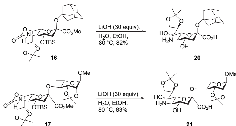
Scheme 2. Hydrolysis of oxazinanone groups in compounds 16 and 17 .
